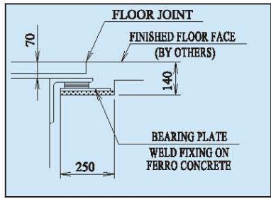
CONCRETE SUPPORT BEAM
